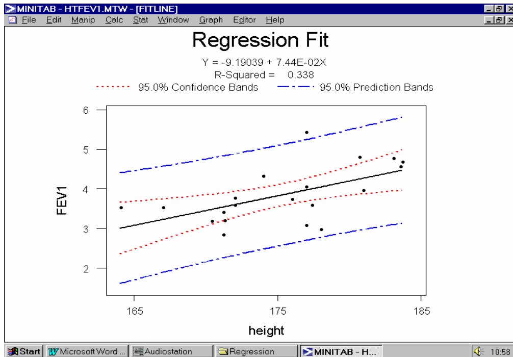
Figure 5: 95% confidence and prediction intervals for the data in figure 1 b)
