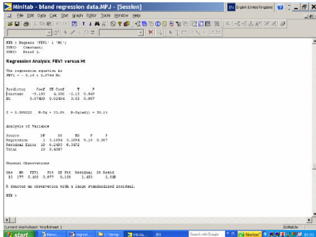
Figure 4: Minitab output after fitting a regression line to the data from Figure 1 b)
