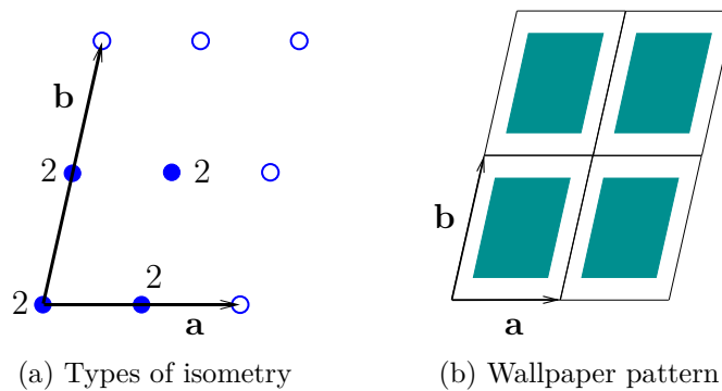
Figure 12: Wallpaper group: type 2222
