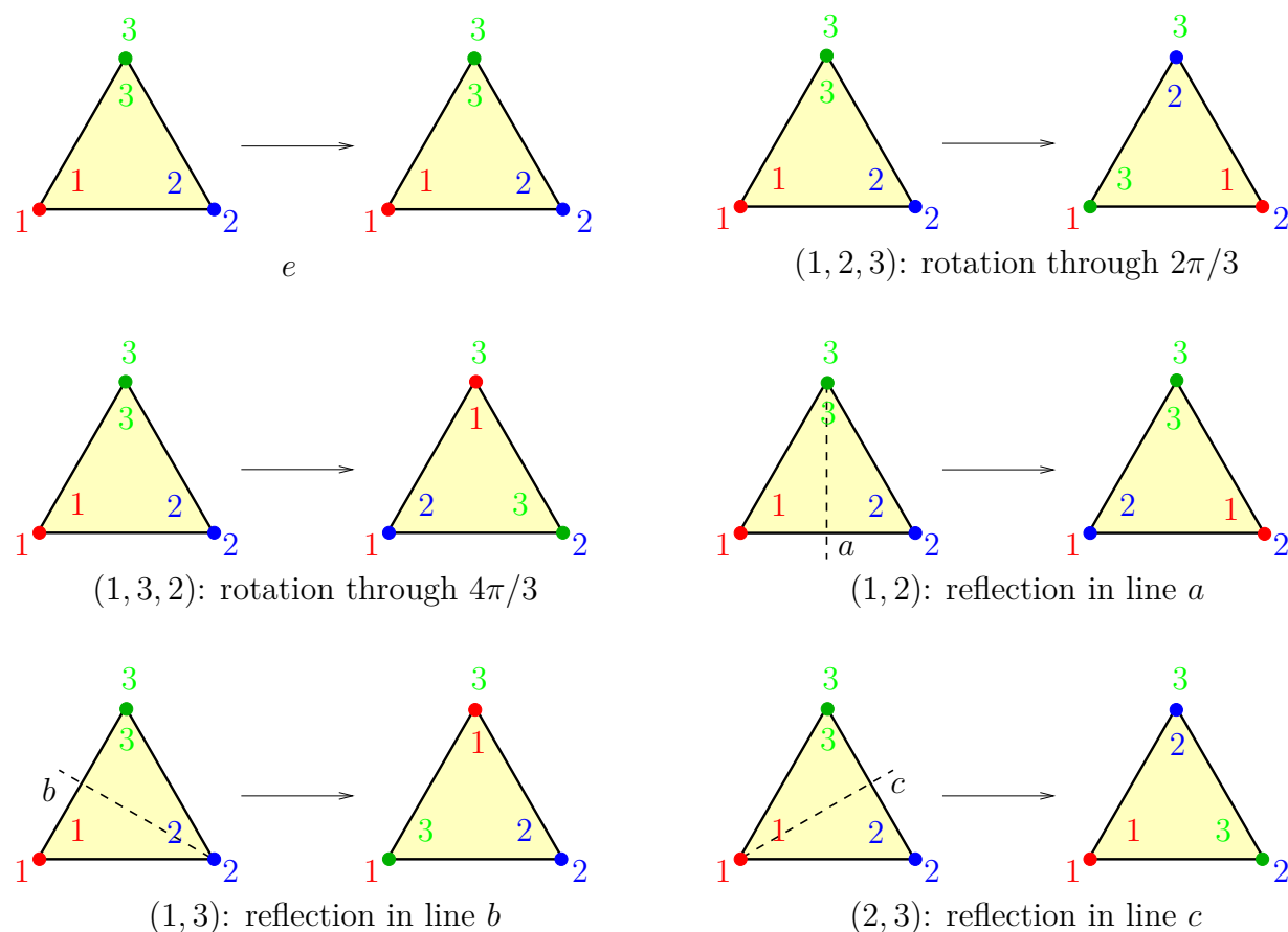
Figure 1: Elements of S_3 as symmetries of a triangle
