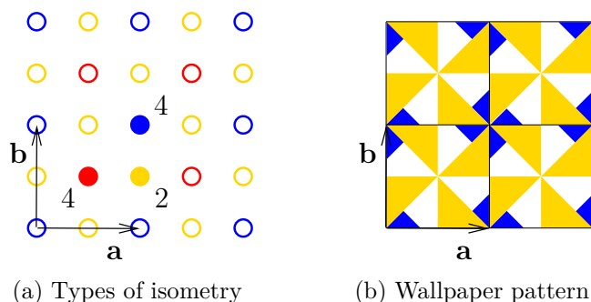
Figure 19: Wallpaper group: type 442
