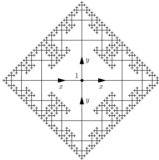
Figure 27: The Cayley graph of the free group F(x, y)
