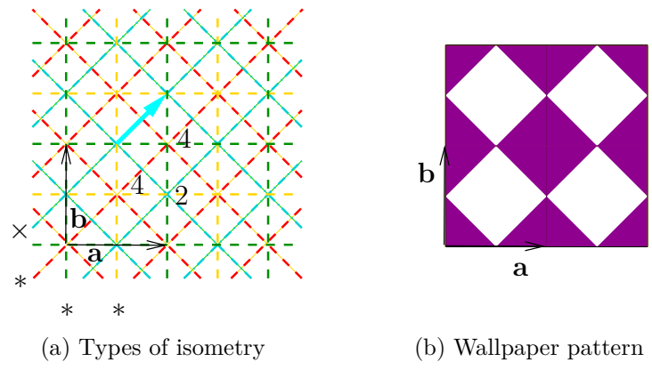
Figure 20: Wallpaper group: type *442
