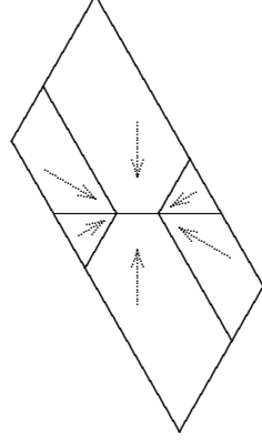
FIGURE 10. Parallelograms in \mathcal{D}'(m, n) .
