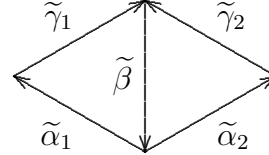
FIGURE 15. Diagram indexing the middle sum in (11).
