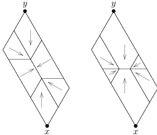
FIGURE 7. Possible labellings of parallelograms.
