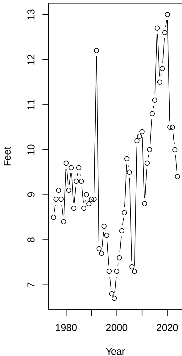
Time series plot of sea-surges
