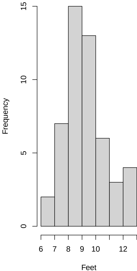
Histogram of sea-surges
