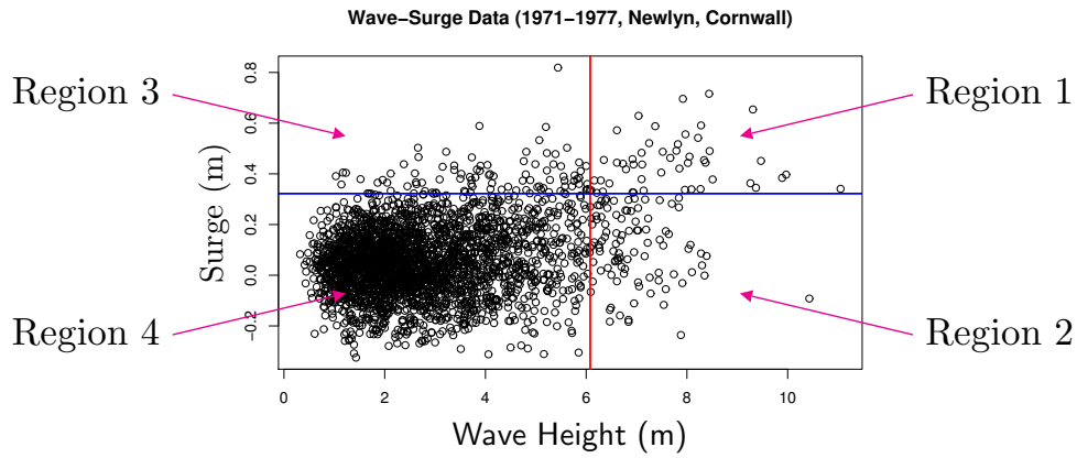
Figure 6.3: Threshold classification of bivariate data.
