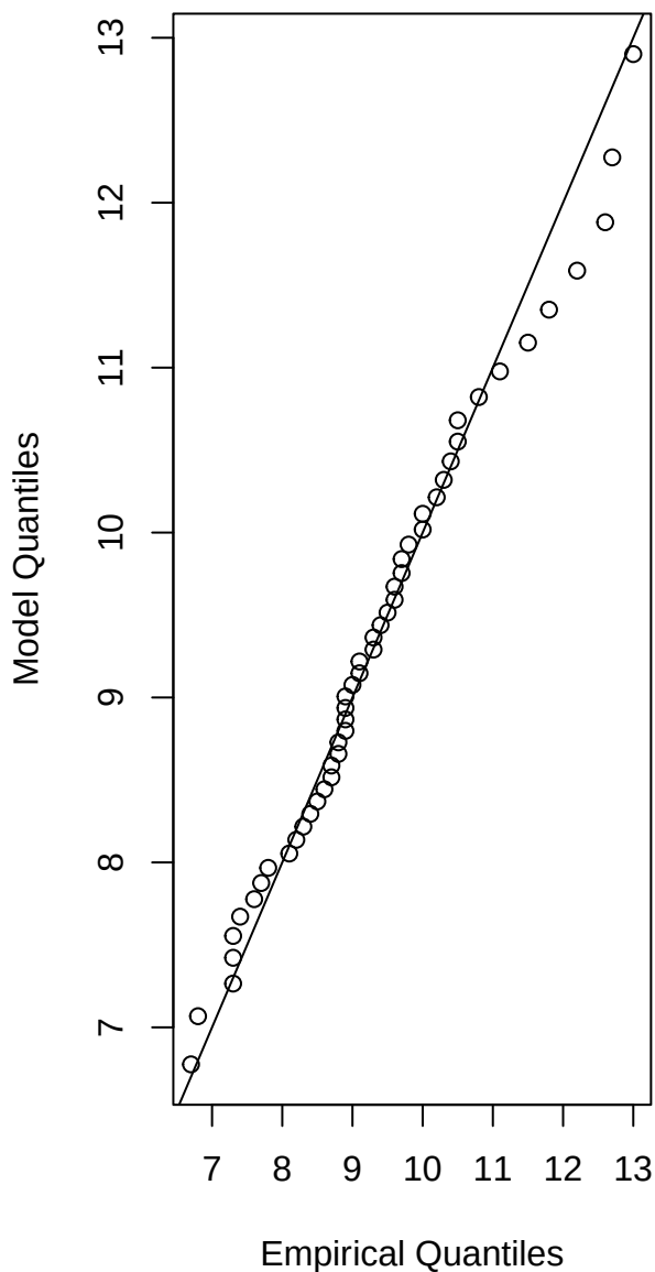
Quantile plot
