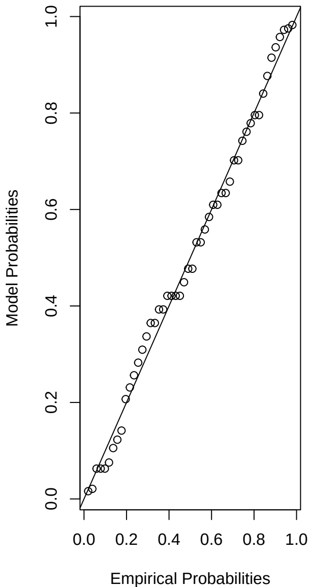
Probability plot
