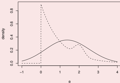
Figure: Plot of two mixture densities: solid is 0.6N(1, 1) + 0.4N(2, 1) ; dashed is 0.9Exp(1) + 0.1N(2, 0.25^2)
