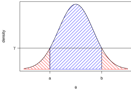
Figure: HDI for \theta
