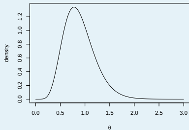
Figure: Posterior density for \theta
