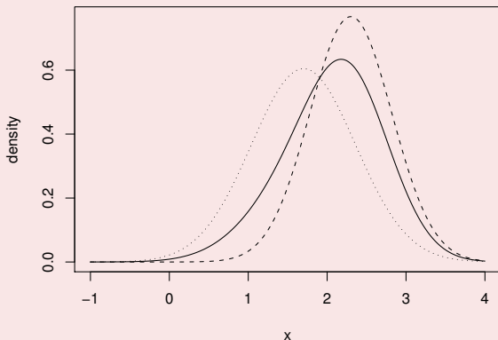
Figure: Plot of the mixture density (solid) with its component densities (survive – dashed; die – dotted)
