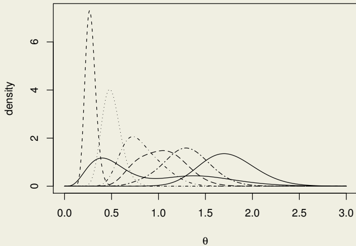
Figure: Plot of the prior distribution (dotted) and various posterior distributions
