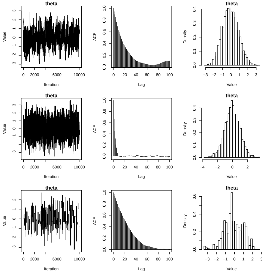
Figure 4.11: Trace plots, autocorrelation plots and histograms of the output from a Metropolis–Hastings sampler using a U(-a, a) random walk proposal. Top row: a = 0.6 ; middle row: a = 6 ; bottom row: a = 60
