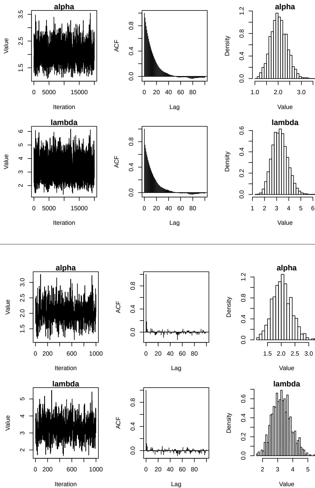
Figure 4.12: Trace plots, autocorrelation plots and histograms of the Metropolis with Gibbs output. Upper plots: all realisations. Lower plots: with burn-in = 10, thin = 20.
