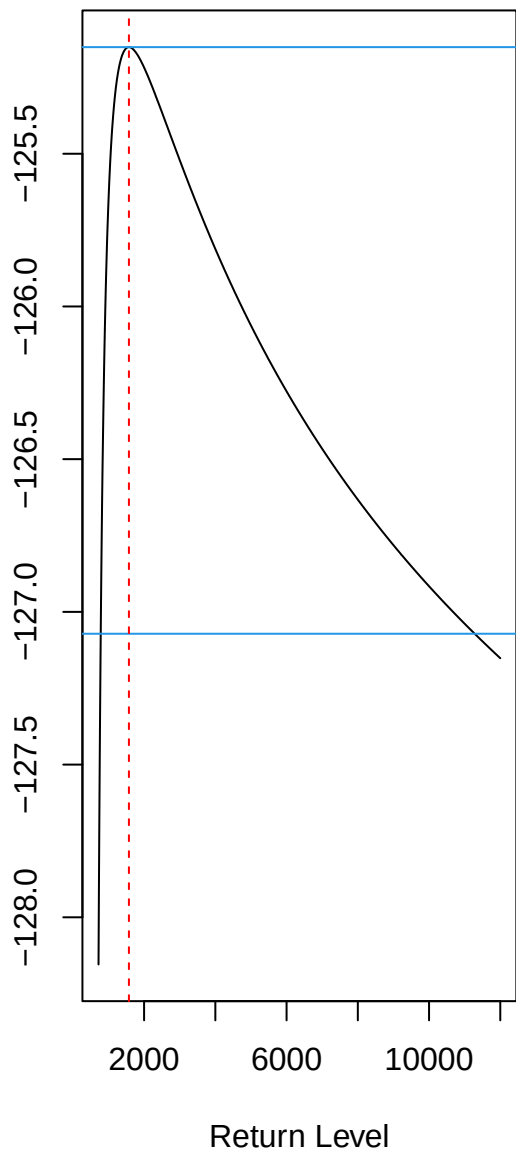
Profile Log-likelihood
