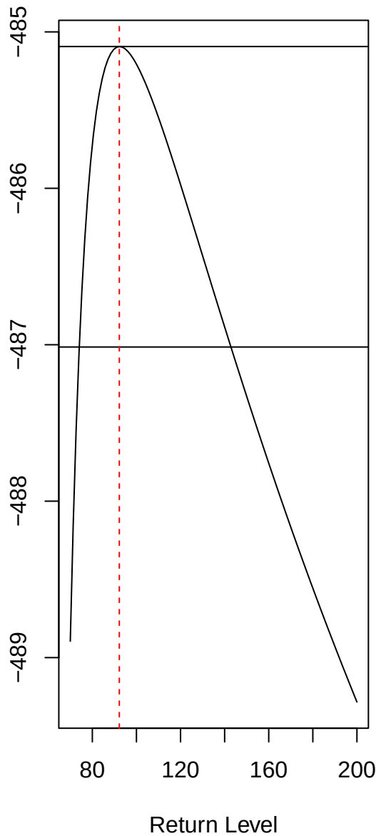
Profile Log-likelihood
