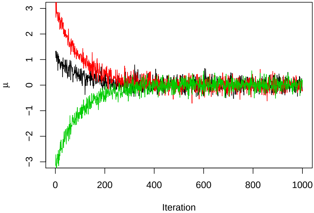
Figure 4.3: Demonstration of burn-in using a Gibbs sampler and three initial values
