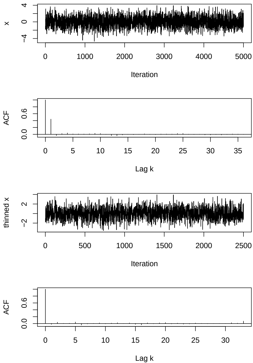
Figure 4.4: Effect of thinning output from a MA(1) process
