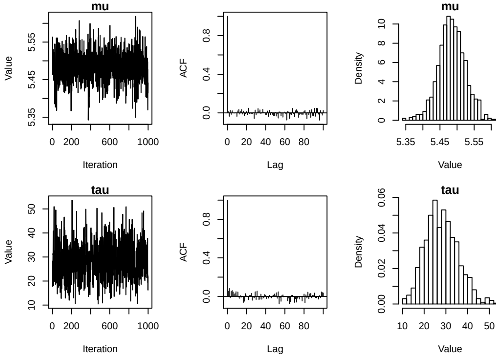
Figure 4.9: Trace plots, autocorrelation plots and histograms of the Gibbs sampler output
