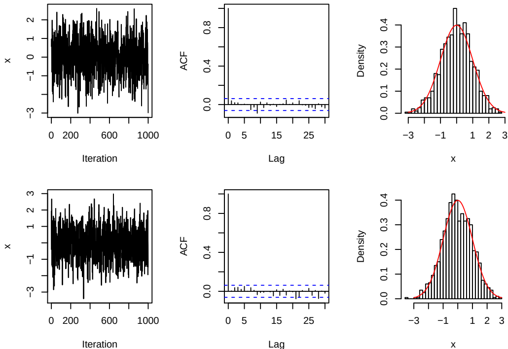
Figure 4.1: Summaries of the 1K realisations from the black box simulator
