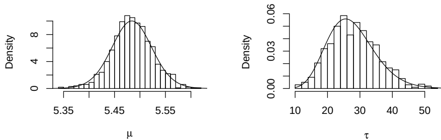
Figure 4.10: Histograms of the Gibbs sampler output and the (known) marginal densities
