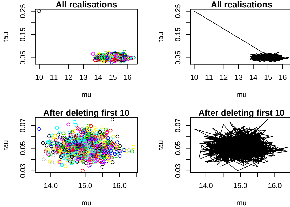
Figure 4.6: Progress of the MCMC scheme
