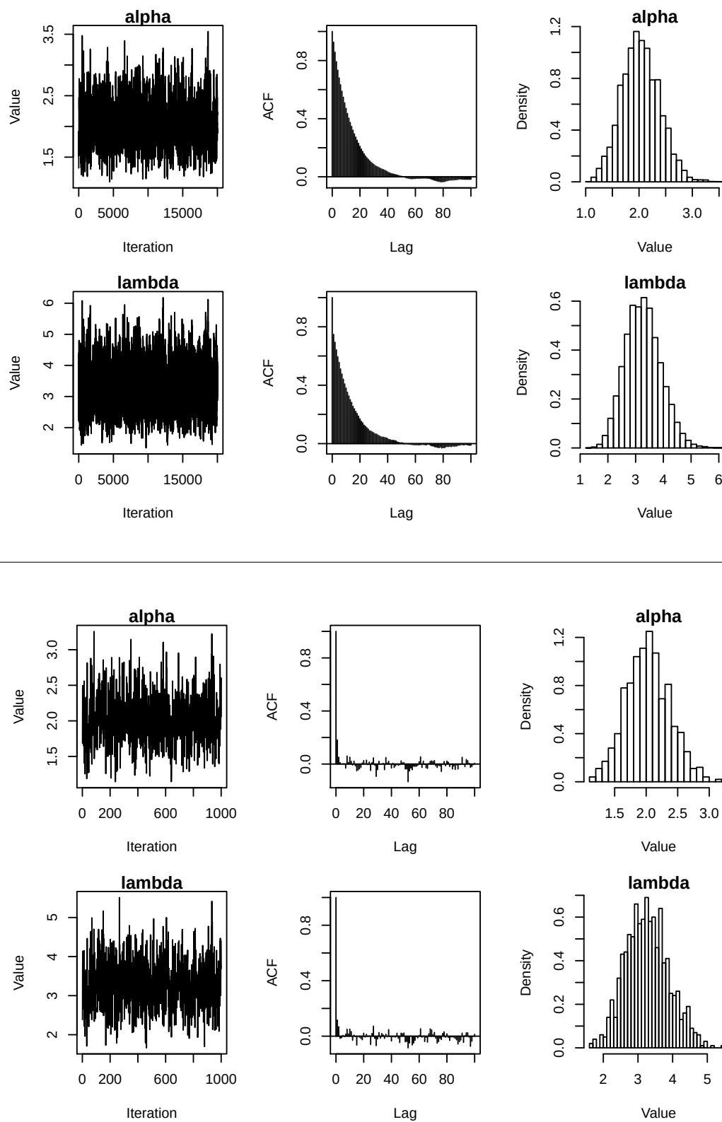
Figure 4.11: Trace plots, autocorrelation plots and histograms of the Metropolis with Gibbs output. Upper plots: all realisations. Lower plots: with burn-in = 10, thin = 20.
