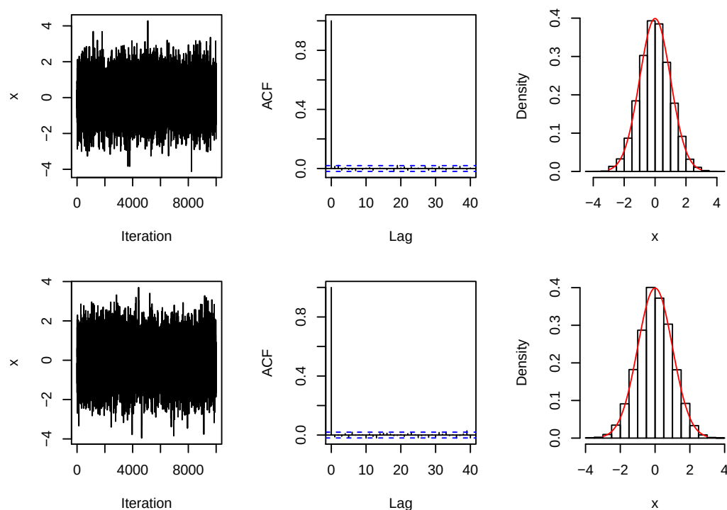
Figure 4.2: Summaries of the 10K realisations from the black box simulator
