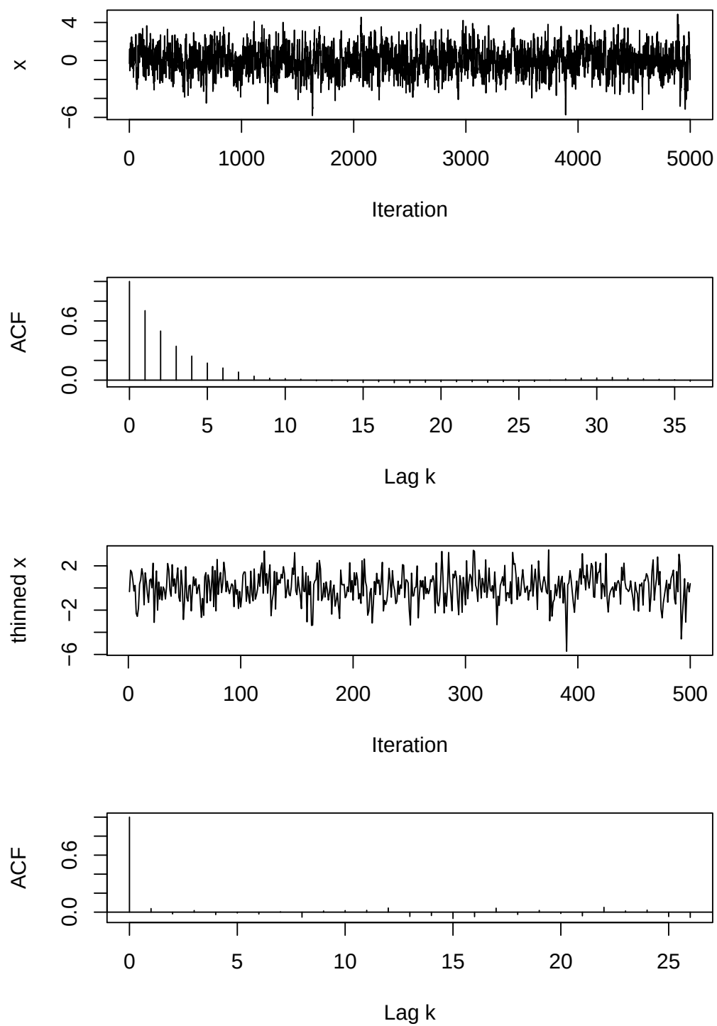
Figure 4.5: Effect of thinning output from a AR(1) process
