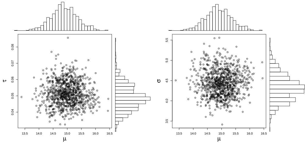
Figure 4.8: Plot of the bivariate posterior sample and their marginal distributions. Left plot: (\mu, \tau)^T ; right plot: (\mu, \sigma)^T .
