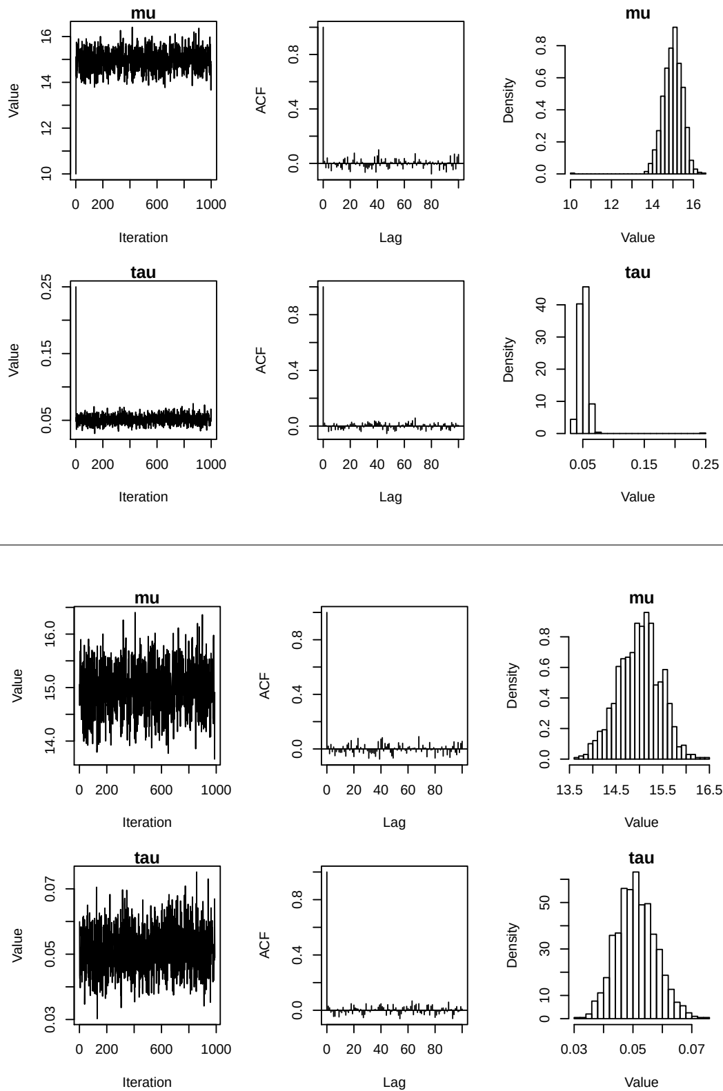
Figure 4.7: Trace plots, autocorrelation plots and histograms of the Gibbs sampler output. Upper plots: all realisations. Lower plots: after deleting the first 10 iterations
