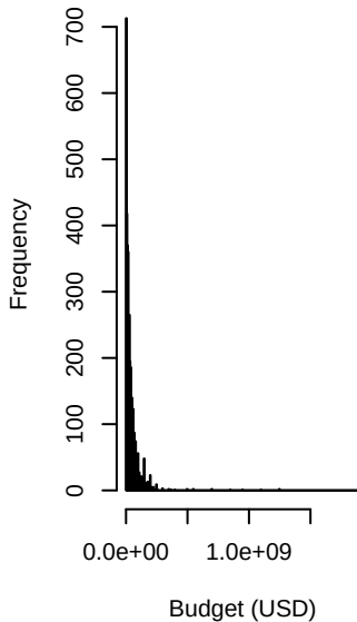
FD rule
