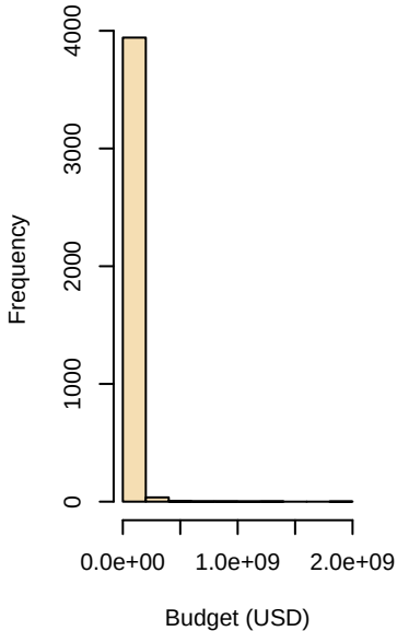
Sturges' rule
